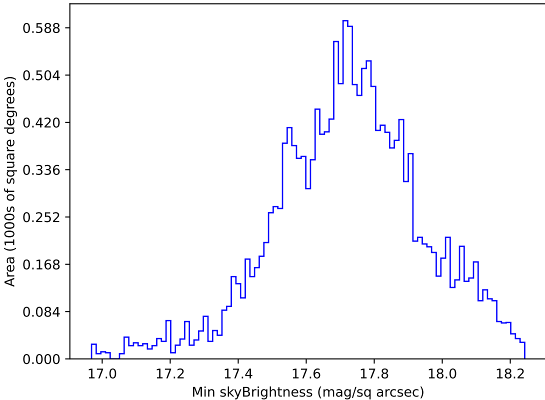
baseline_v2.1_10yrs WFD z band: Min skyBrightness
