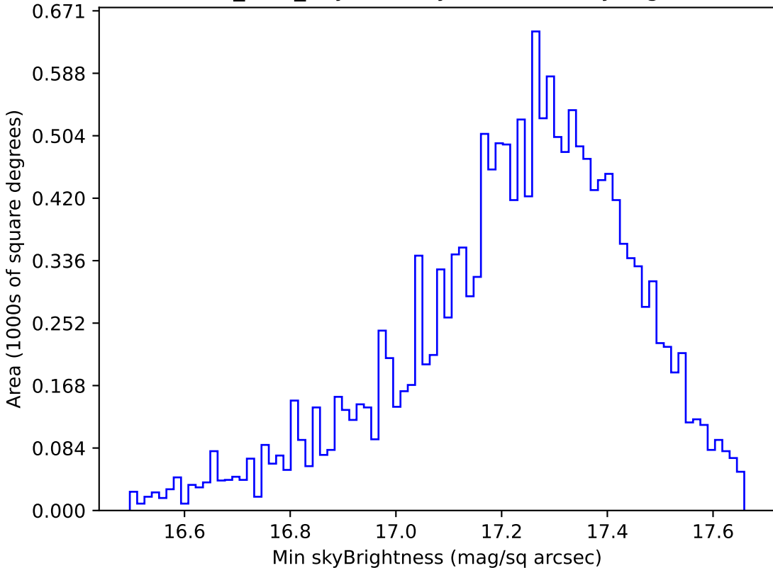
baseline_v2.1_10yrs WFD y band: Min skyBrightness
