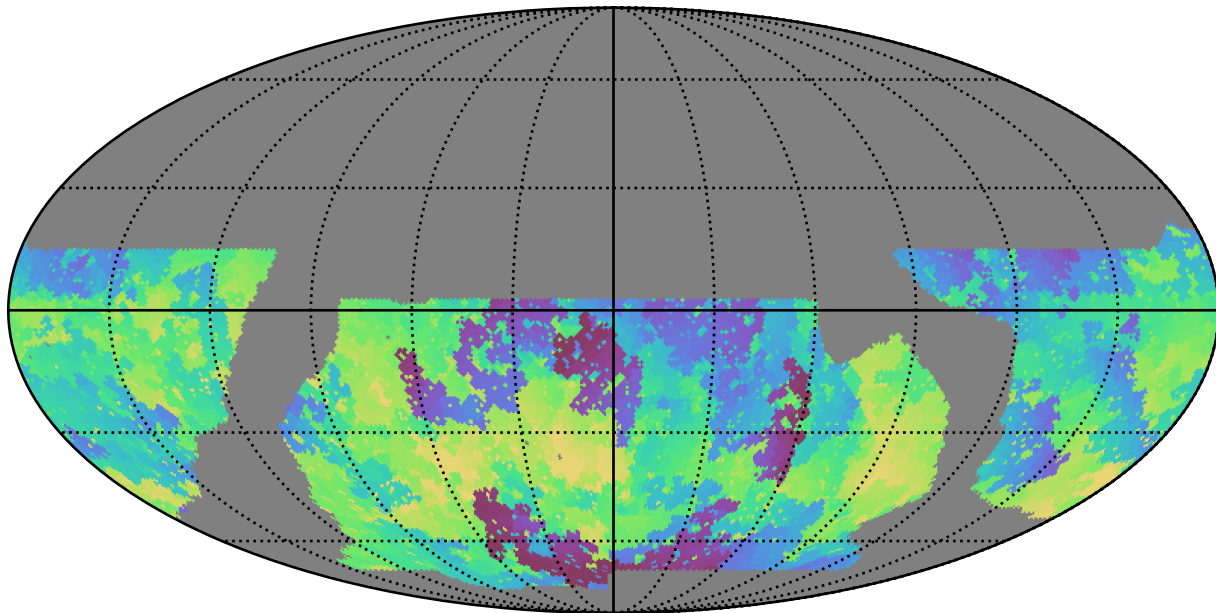
baseline_v2.1_10yrs WFD u band: Min skyBrightness
