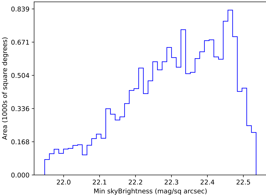
baseline_v2.1_10yrs WFD u band: Min skyBrightness
