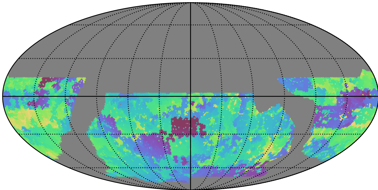
baseline_v2.1_10yrs WFD r band: Min skyBrightness
