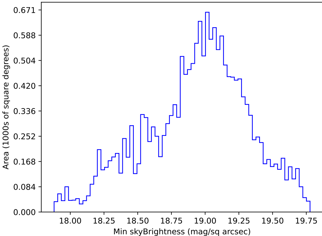
baseline_v2.1_10yrs WFD r band: Min skyBrightness
