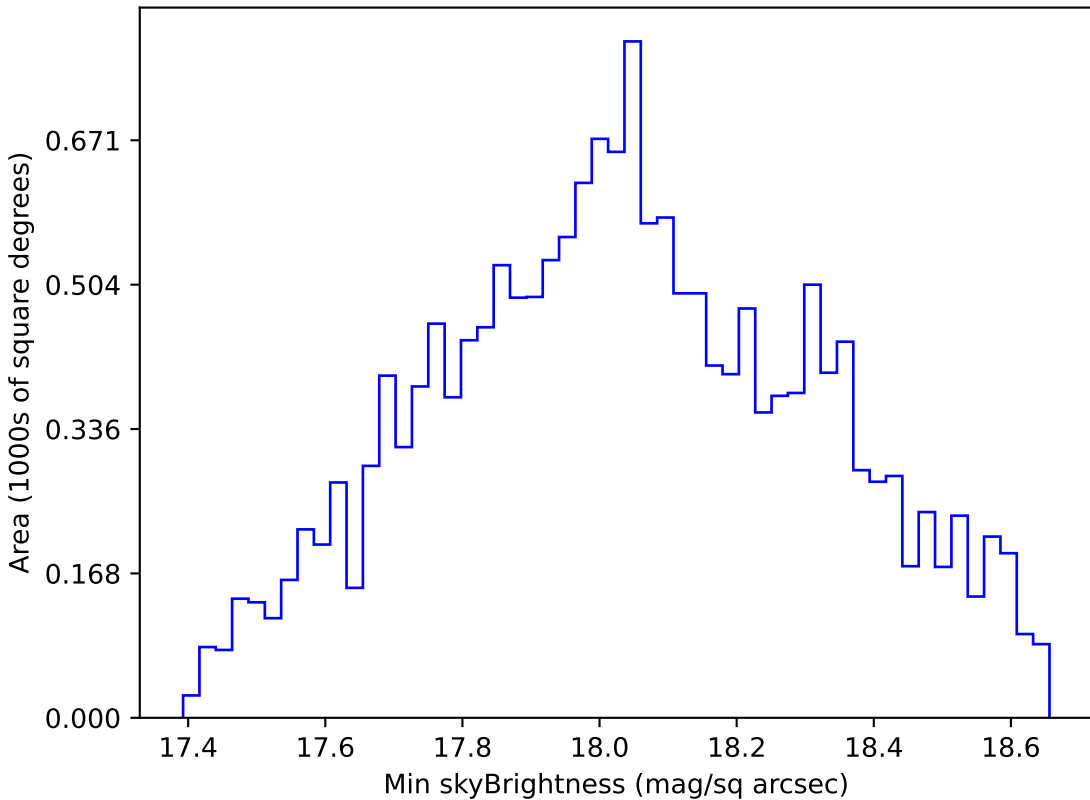
baseline_v2.1_10yrs WFD i band: Min skyBrightness
