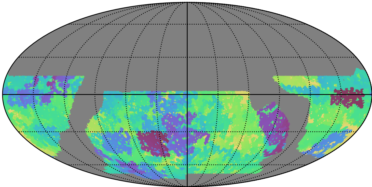
baseline_v2.1_10yrs WFD g band: Min skyBrightness
