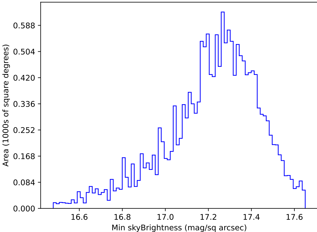
baseline_v2.1_10yrs WFD all bands: Min skyBrightness
