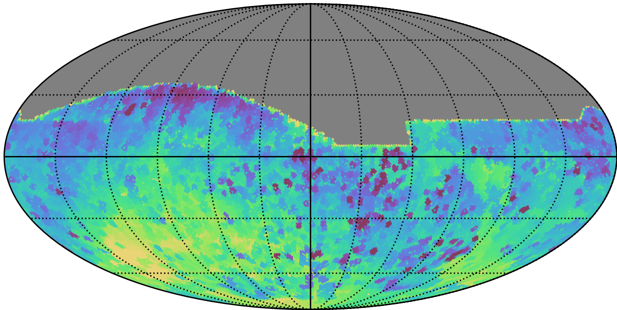
baseline_v2.1_10yrs All sky z band: Min skyBrightness
