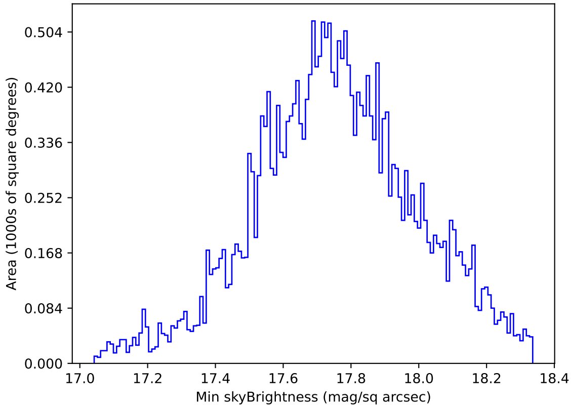
baseline_v2.1_10yrs All sky z band: Min skyBrightness
