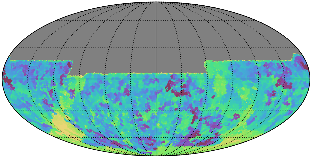
baseline_v2.1_10yrs All sky y band: Min skyBrightness
