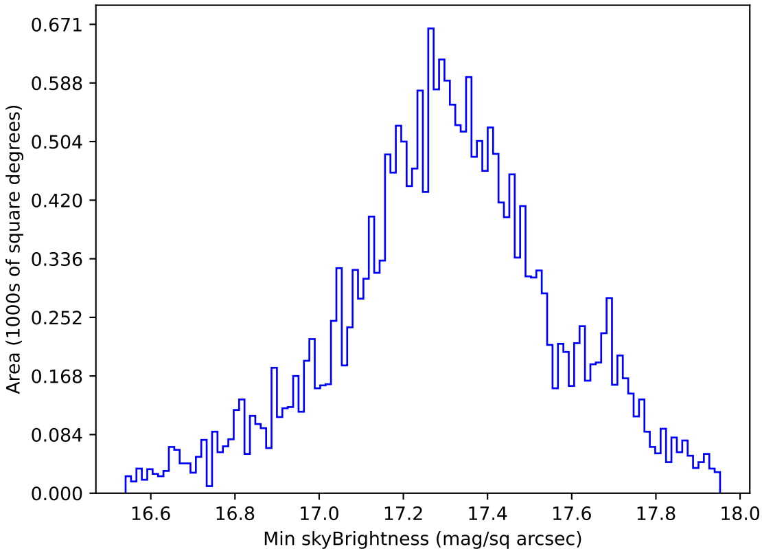
baseline_v2.1_10yrs All sky y band: Min skyBrightness
