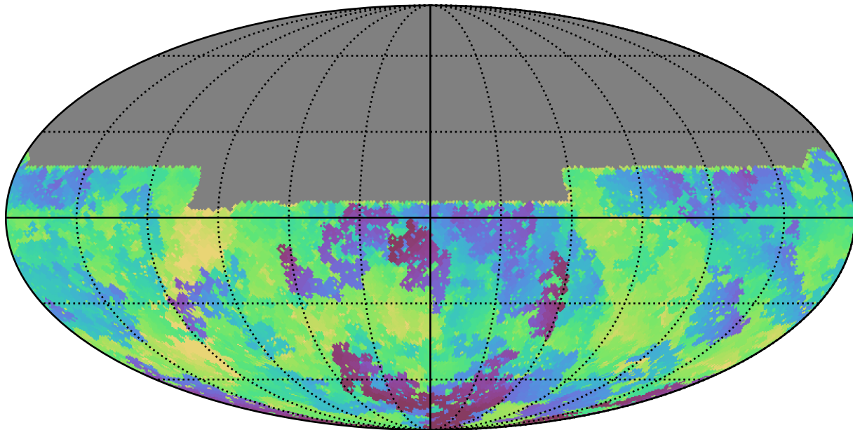
baseline_v2.1_10yrs All sky u band: Min skyBrightness
