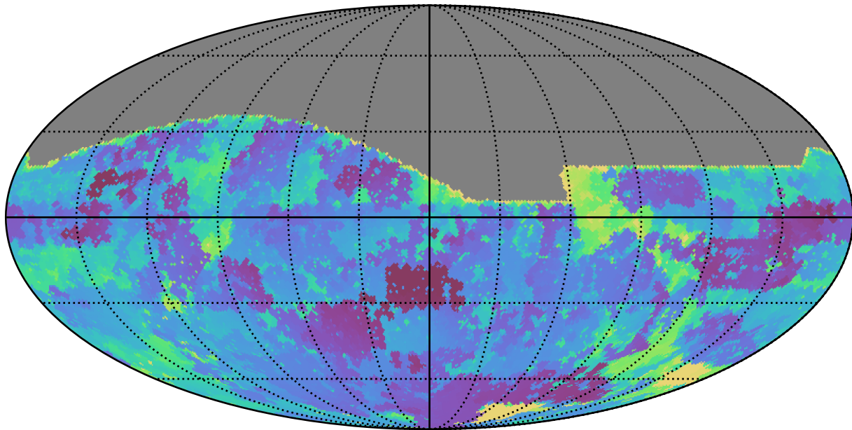
baseline_v2.1_10yrs All sky r band: Min skyBrightness
