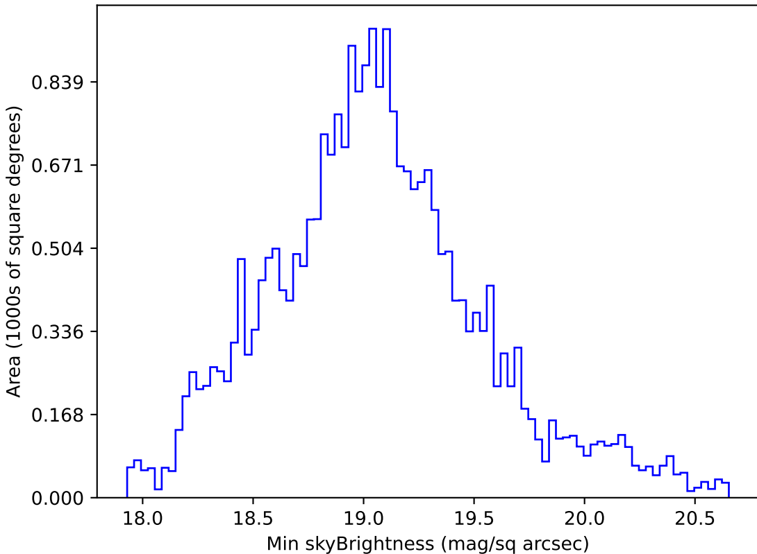
baseline_v2.1_10yrs All sky r band: Min skyBrightness
