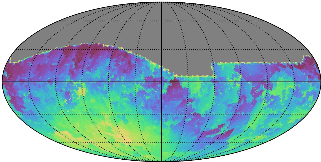
baseline_v2.1_10yrs All sky i band: Min skyBrightness
