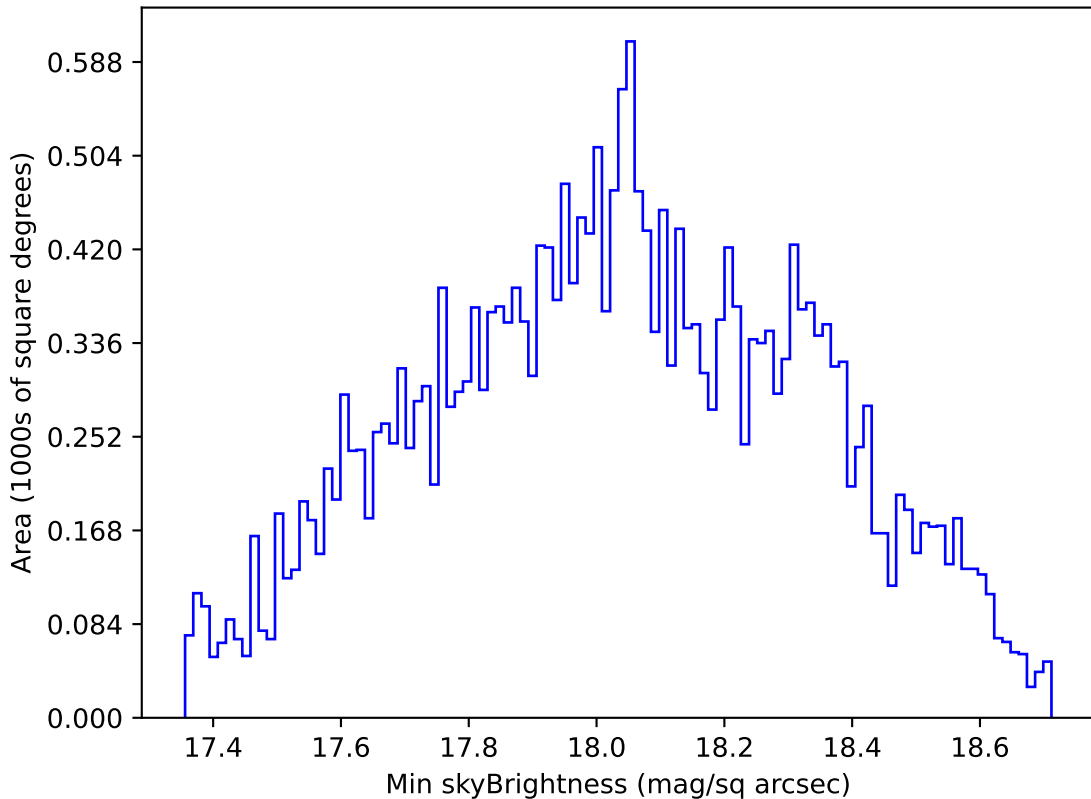
baseline_v2.1_10yrs All sky i band: Min skyBrightness
