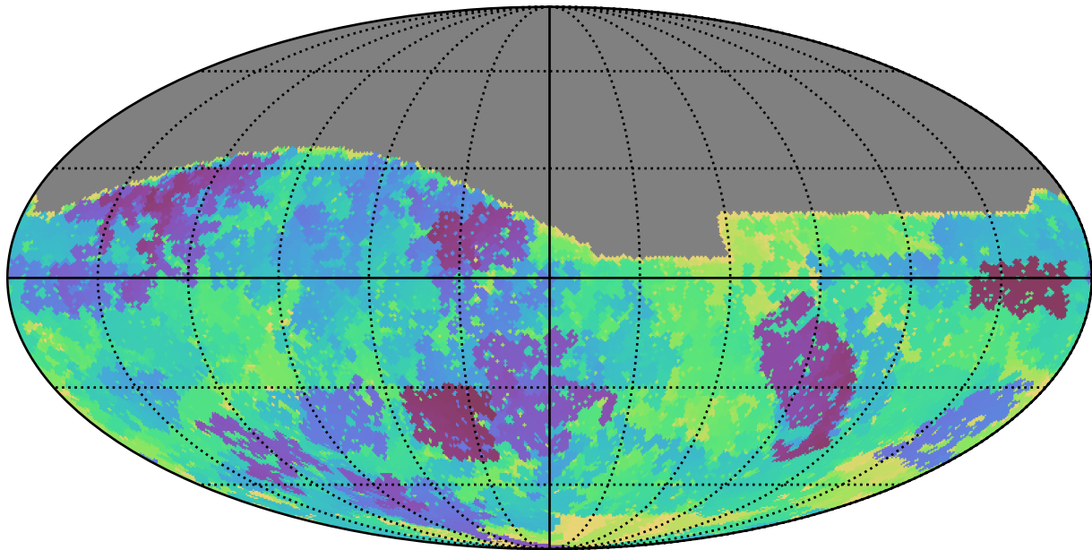
baseline_v2.1_10yrs All sky g band: Min skyBrightness
