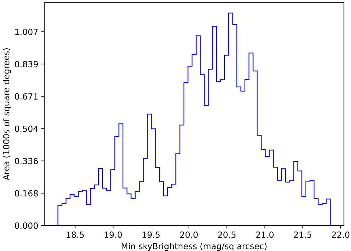
baseline_v2.1_10yrs All sky g band: Min skyBrightness
