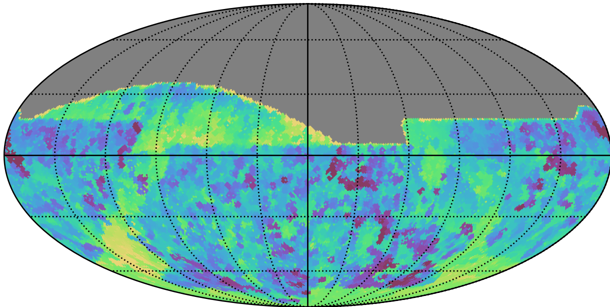
baseline_v2.1_10yrs All sky all bands: Min skyBrightness
