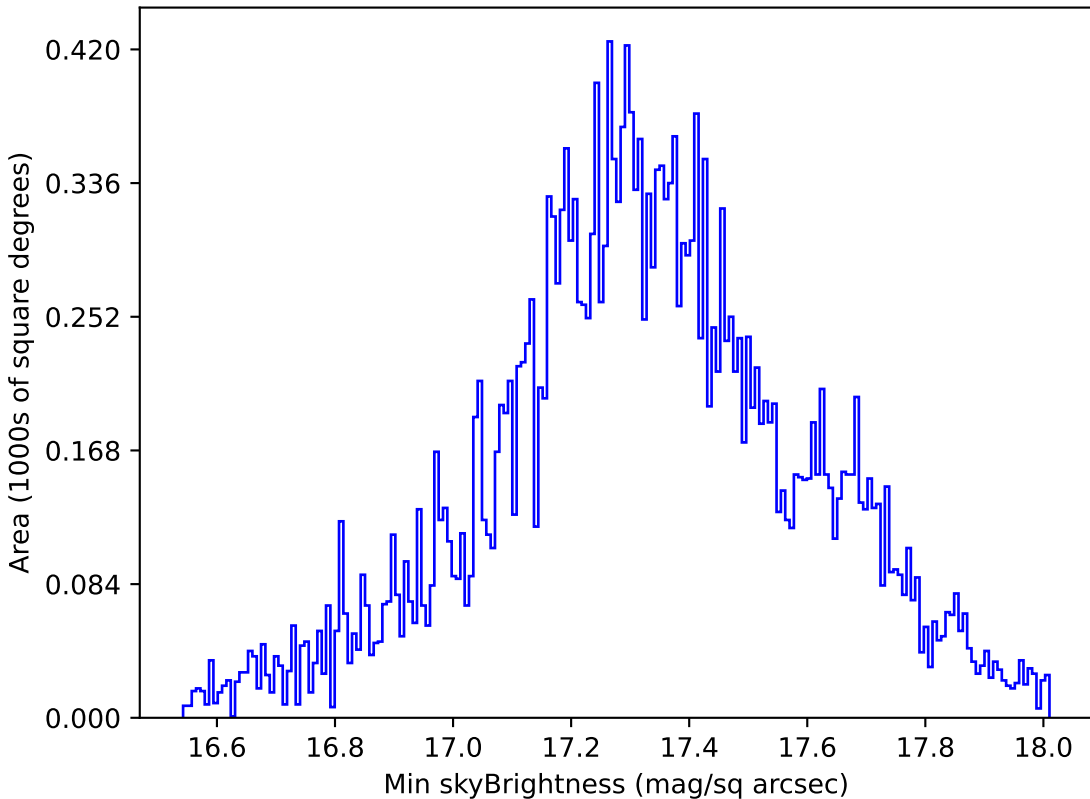
baseline_v2.1_10yrs All sky all bands: Min skyBrightness
