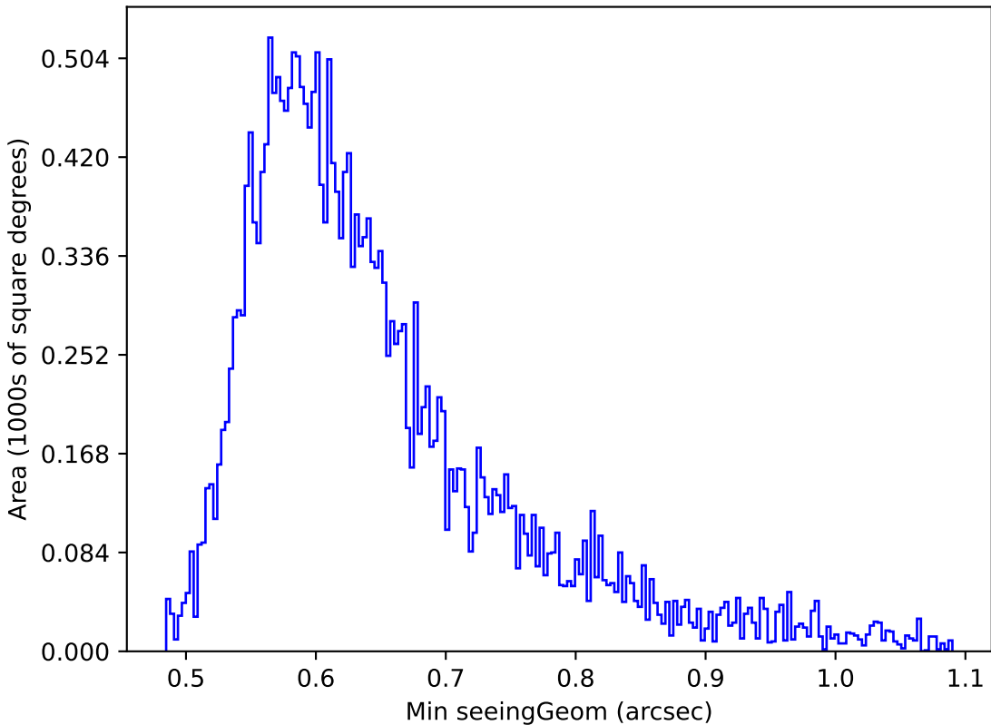
baseline_v2.1_10yrs Yr 1 z band: Min seeingGeom
