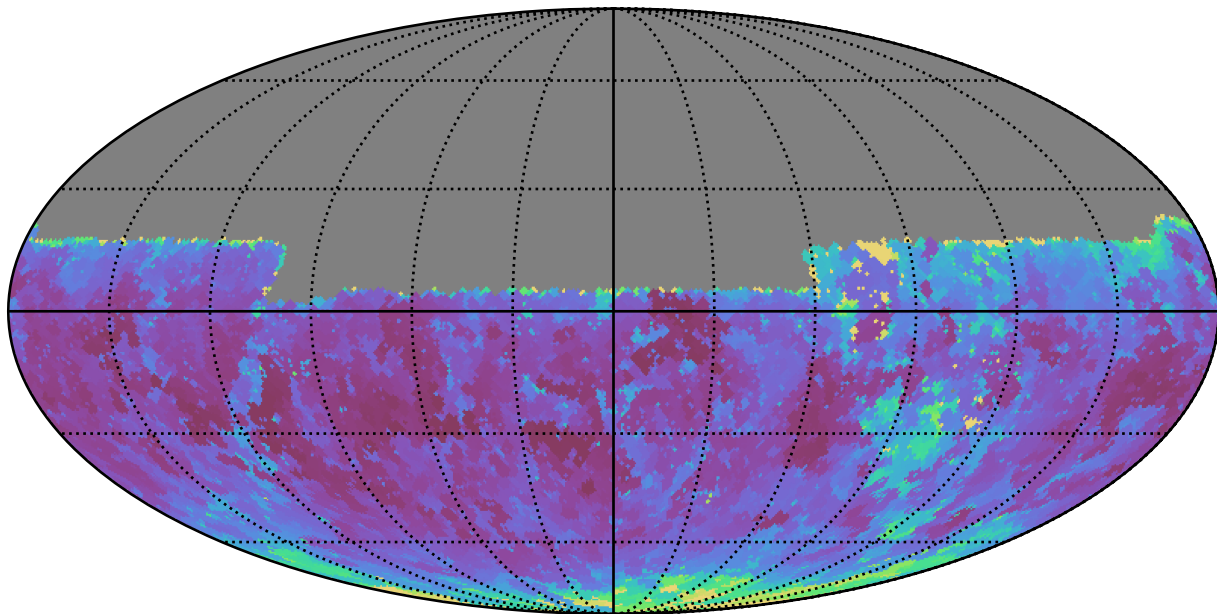
baseline_v2.1_10yrs Yr 1 y band: Min seeingGeom
