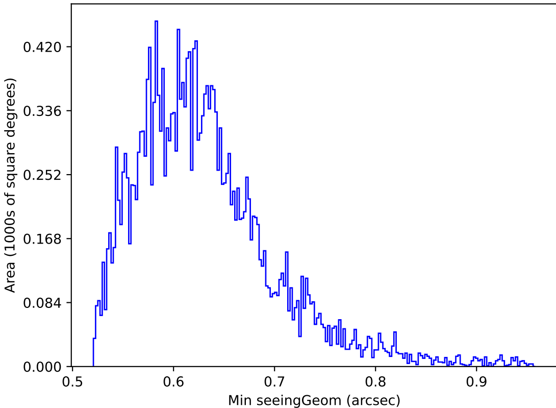
baseline_v2.1_10yrs Yr 1 y band: Min seeingGeom
