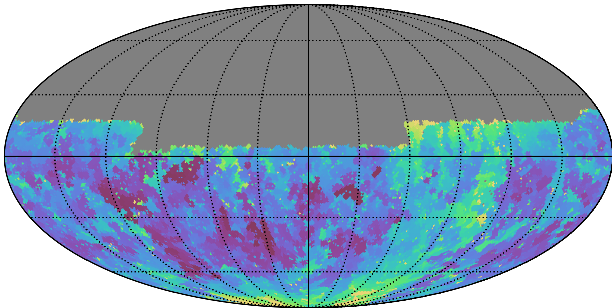
baseline_v2.1_10yrs Yr 1 u band: Min seeingGeom
