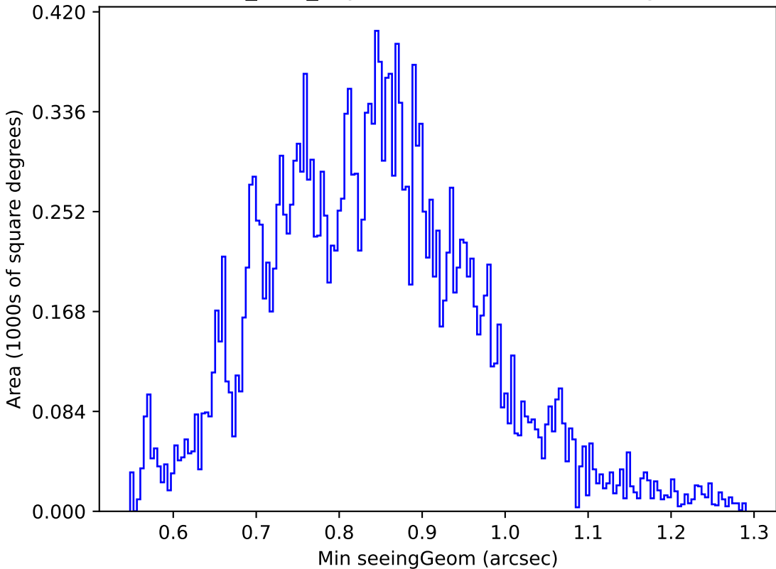
baseline_v2.1_10yrs Yr 1 u band: Min seeingGeom
