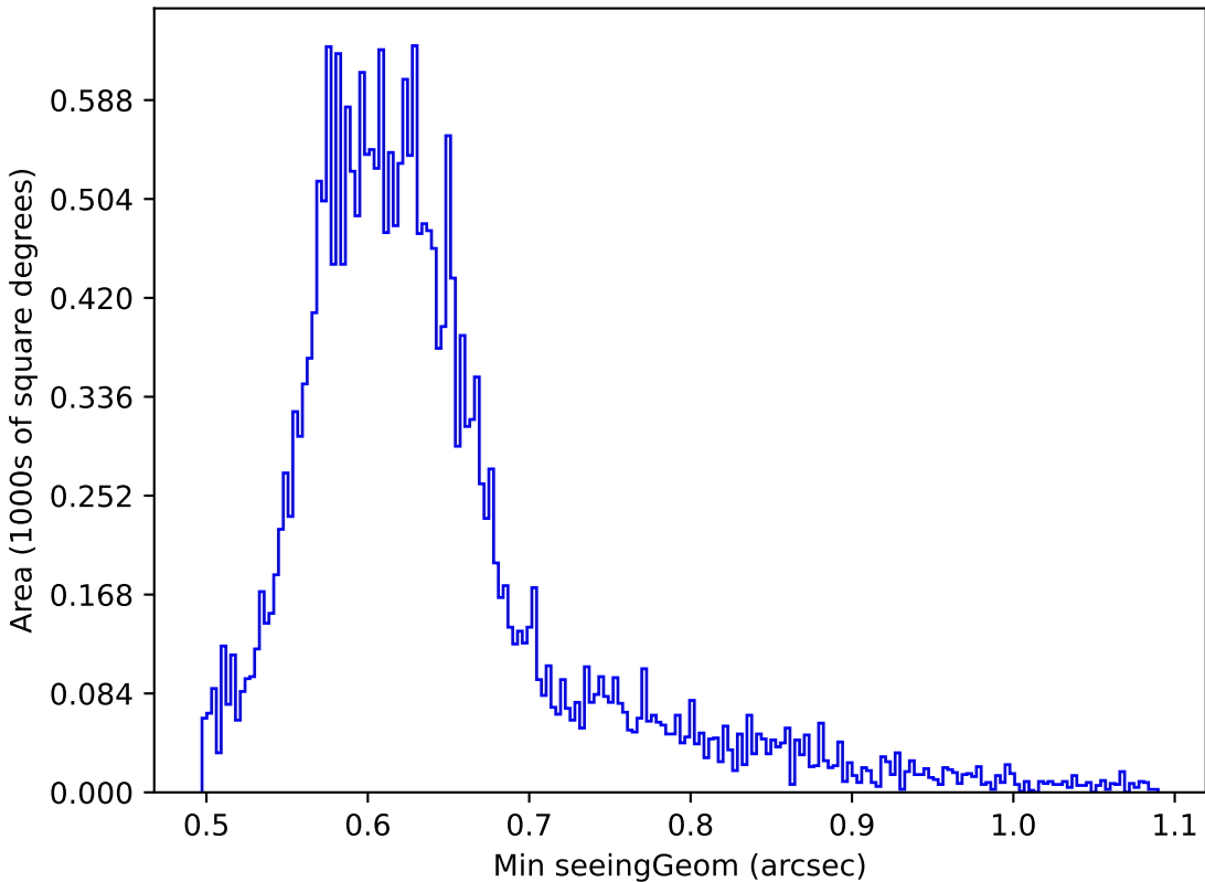
baseline_v2.1_10yrs Yr 1 r band: Min seeingGeom
