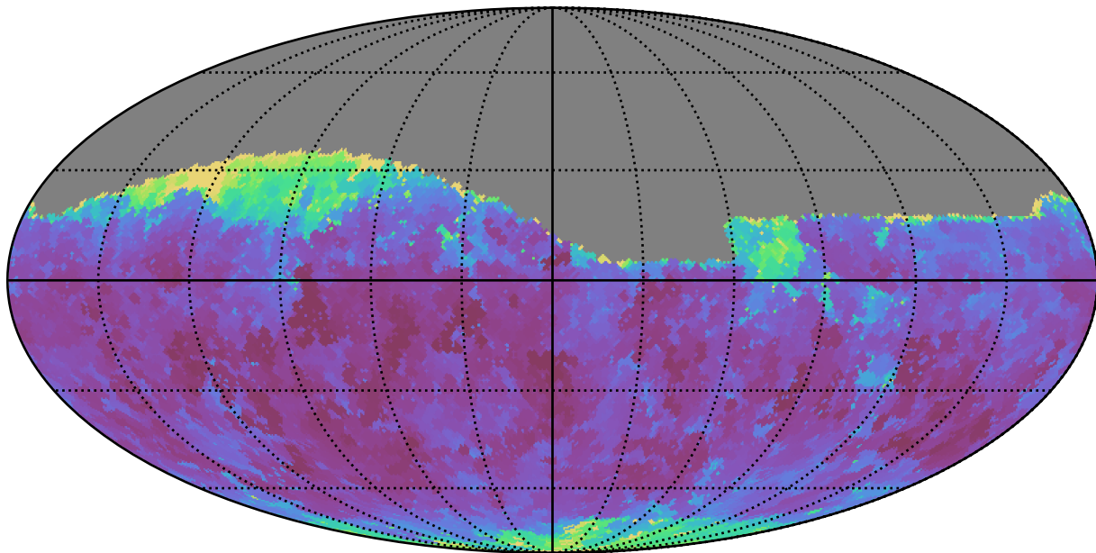
baseline_v2.1_10yrs Yr 1 i band: Min seeingGeom
