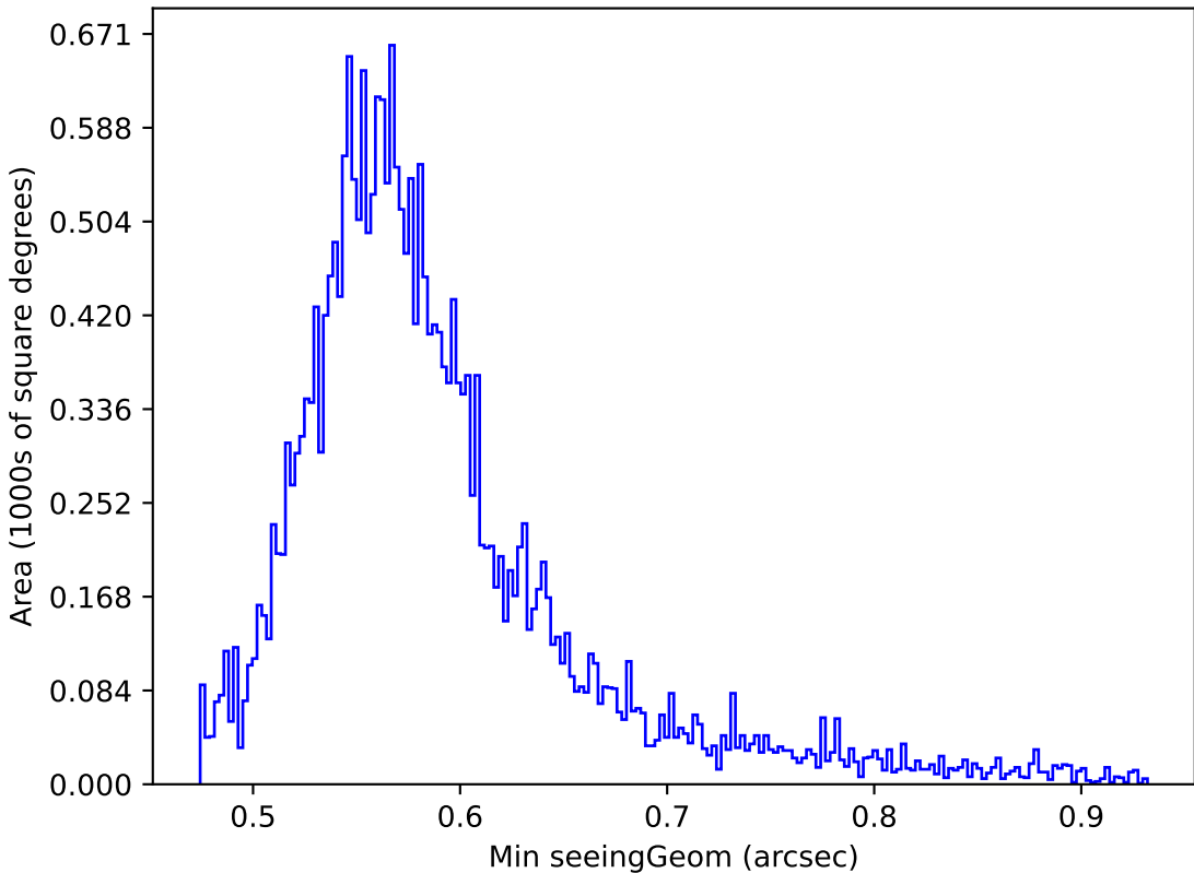
baseline_v2.1_10yrs Yr 1 all bands: Min seeingGeom
