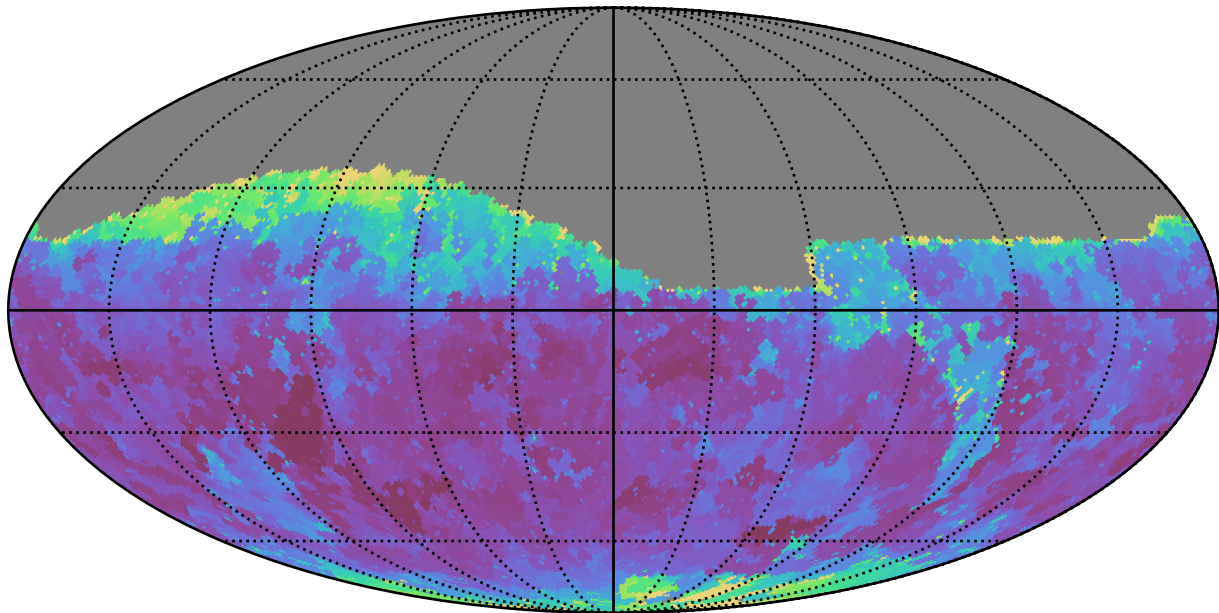
baseline_v2.1_10yrs Yr 1 z band: Min seeingEff
