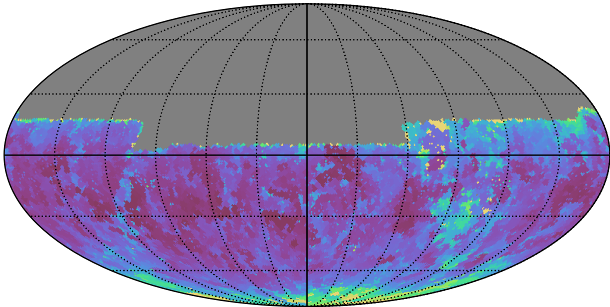
baseline_v2.1_10yrs Yr 1 y band: Min seeingEff
