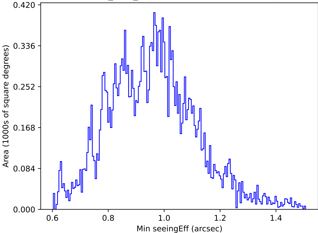
baseline_v2.1_10yrs Yr 1 u band: Min seeingEff
