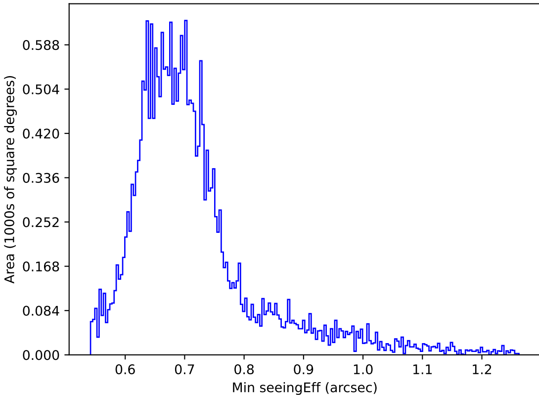
baseline_v2.1_10yrs Yr 1 r band: Min seeingEff
