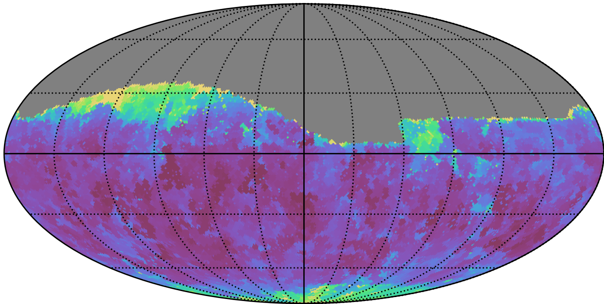
baseline_v2.1_10yrs Yr 1 i band: Min seeingEff
