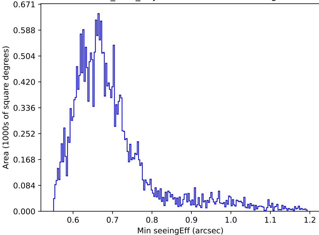
baseline_v2.1_10yrs Yr 1 i band: Min seeingEff
