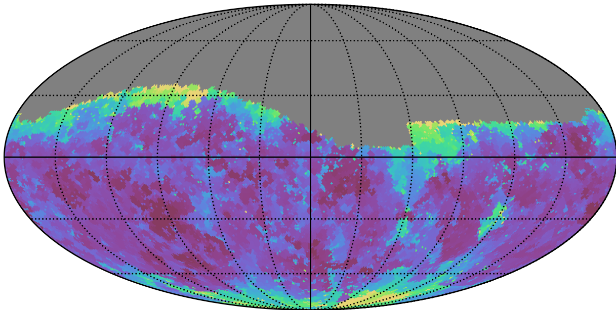
baseline_v2.1_10yrs Yr 1 g band: Min seeingEff
