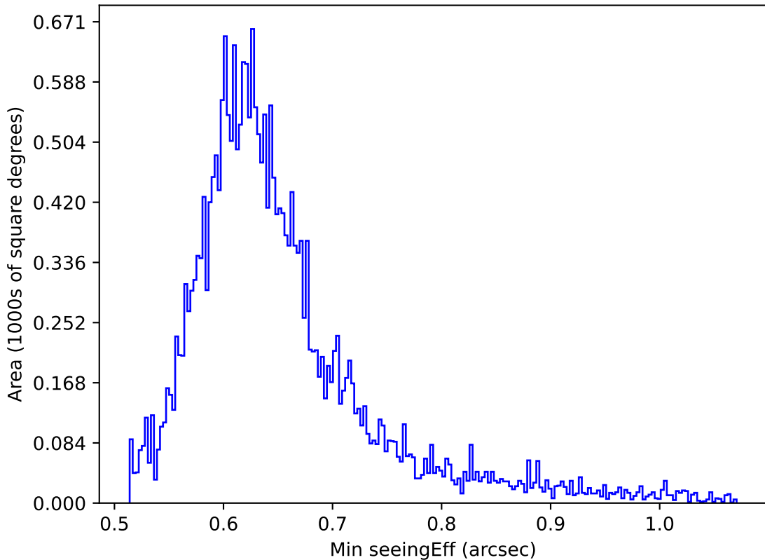
baseline_v2.1_10yrs Yr 1 all bands: Min seeingEff
