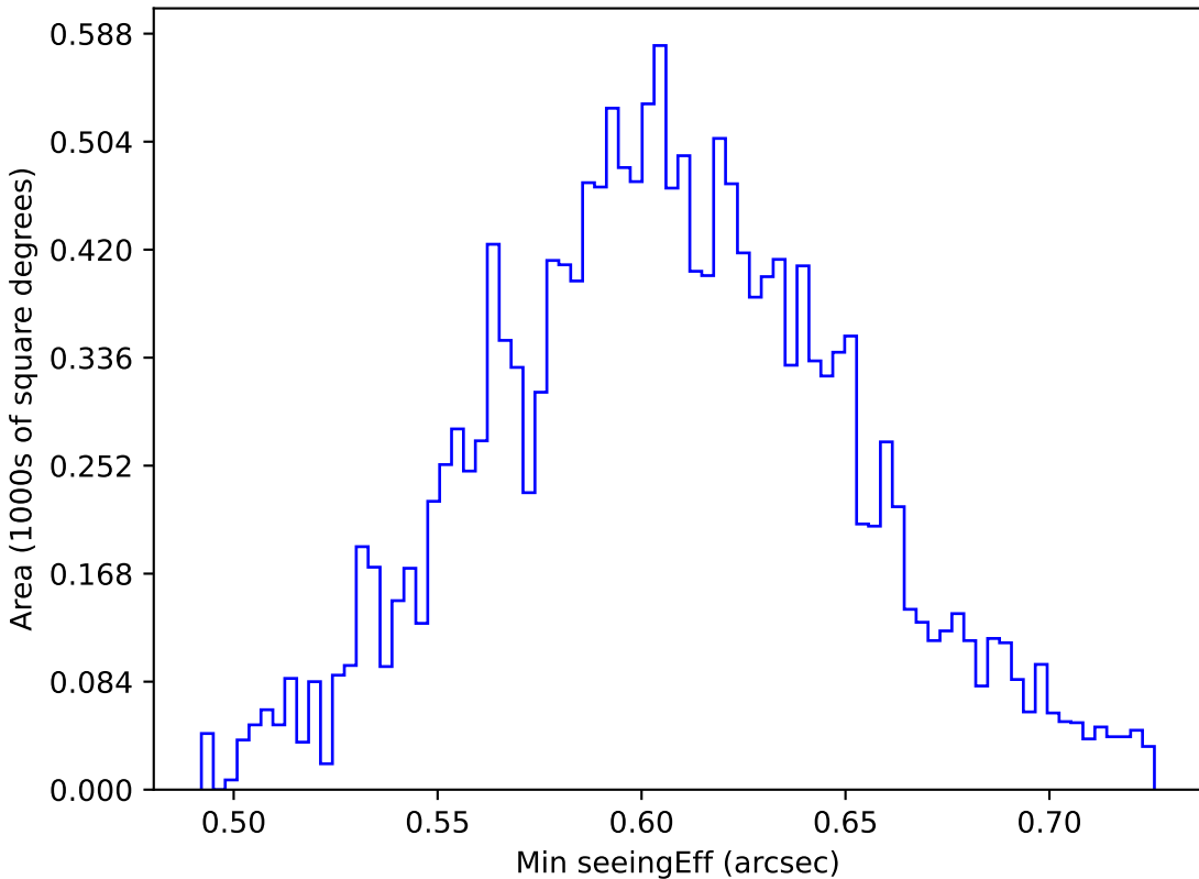
baseline_v2.1_10yrs WFD z band: Min seeingEff
