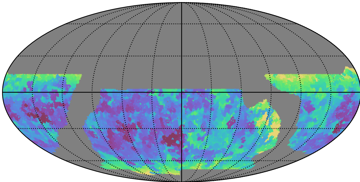
baseline_v2.1_10yrs WFD y band: Min seeingEff
