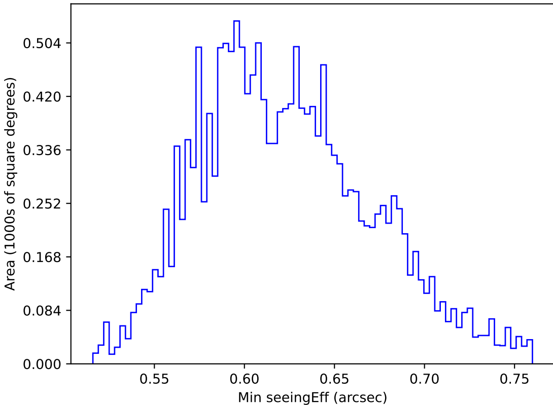
baseline_v2.1_10yrs WFD y band: Min seeingEff
