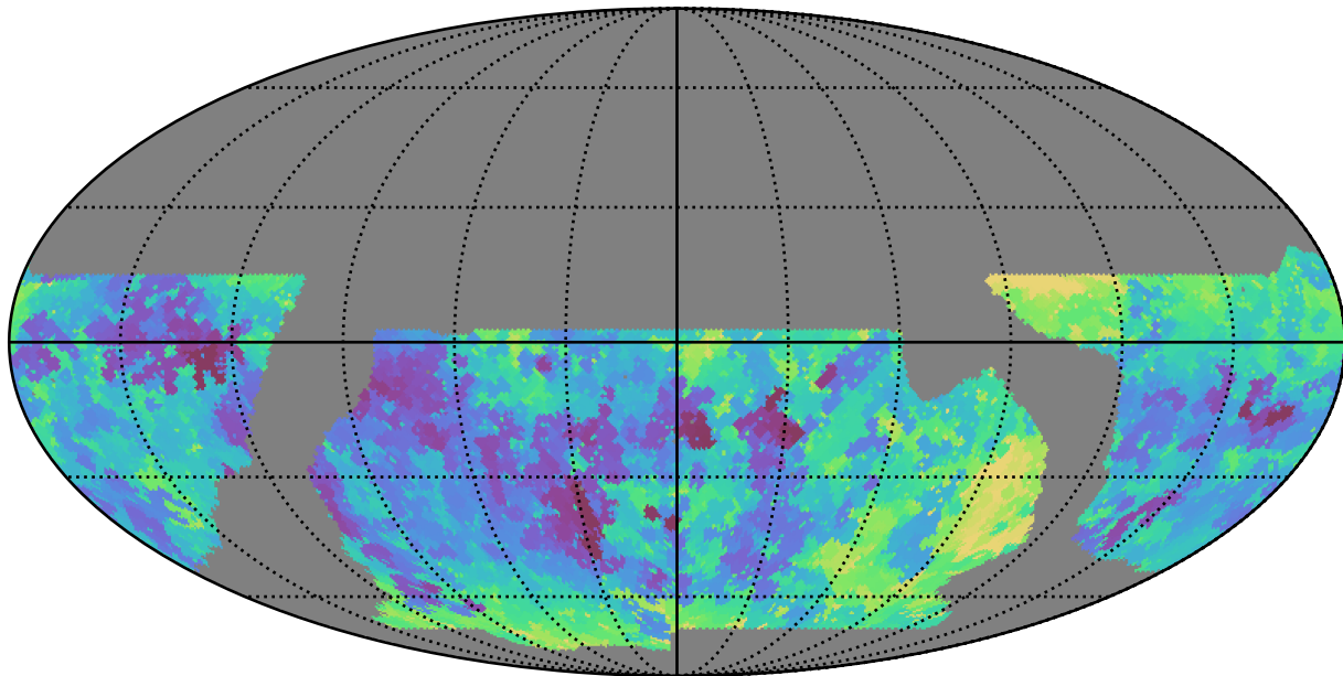
baseline_v2.1_10yrs WFD u band: Min seeingEff
