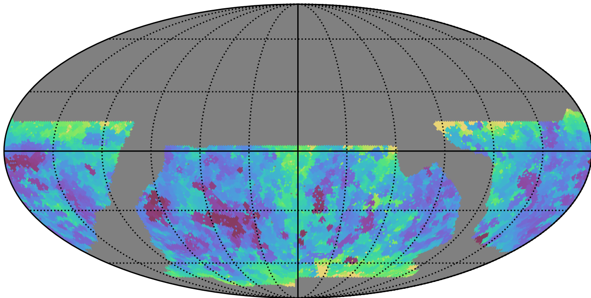
baseline_v2.1_10yrs WFD g band: Min seeingEff
