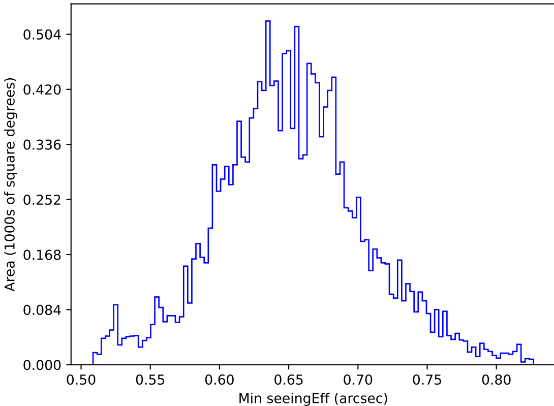
baseline_v2.1_10yrs WFD g band: Min seeingEff
