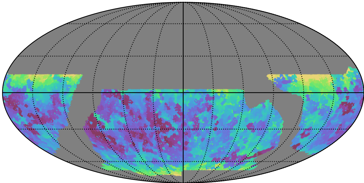
baseline_v2.1_10yrs WFD all bands: Min seeingEff
