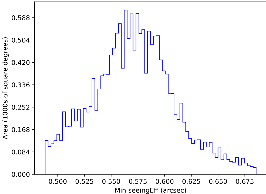
baseline_v2.1_10yrs WFD all bands: Min seeingEff
