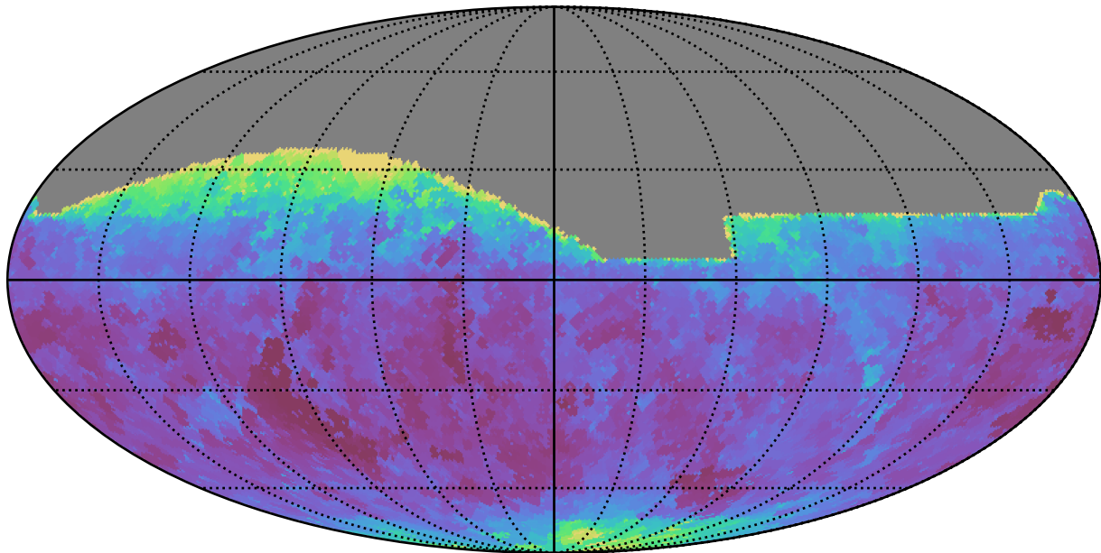
baseline_v2.1_10yrs All sky z band: Min seeingEff
