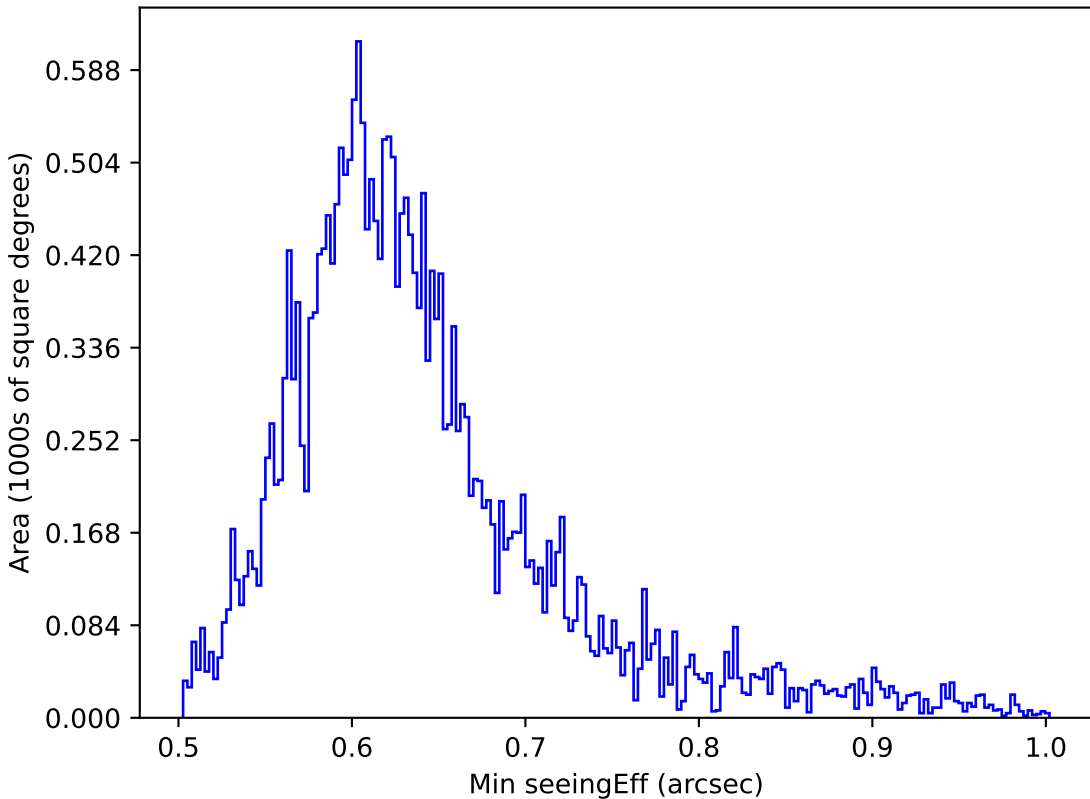
baseline_v2.1_10yrs All sky z band: Min seeingEff
