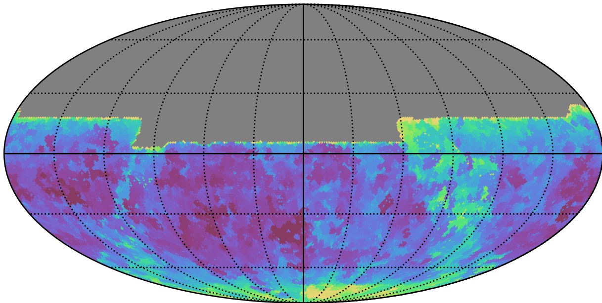
baseline_v2.1_10yrs All sky y band: Min seeingEff
