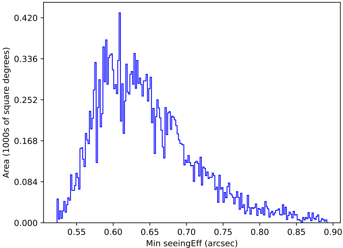
baseline_v2.1_10yrs All sky y band: Min seeingEff
